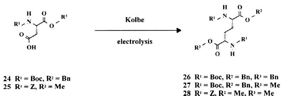
Scheme 4: Synthesis of 2,5-diaminoadipic acid derivatives by Kolbe electrolysis
