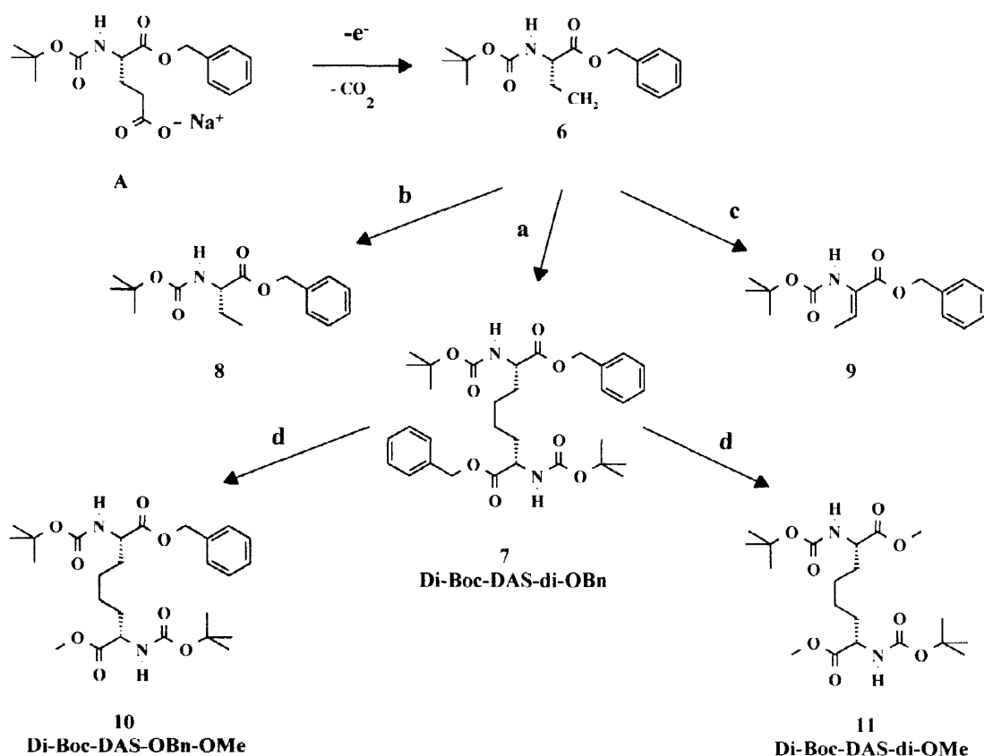
Scheme 2: Mechanism and side products of the Kolbe electrolysis of Boc-Glu-OBn
