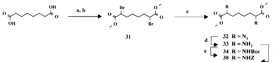
Scheme 5: Preparation of optically inactive 2,7-diaminosuberic acid derivatives: a) SOCl_2 , reflux, 1.5h; b) i) Br_2 , 45–50°C, 50h; ii) MeOH; c) NaN_3 , MeOH, reflux, 17h; d) H_2 , Pd/C, dioxane; e) (Boc)_2O , dioxane/water; f) benzyloxycarbonyl chloride, NaHCO_3 , dioxane/water.
