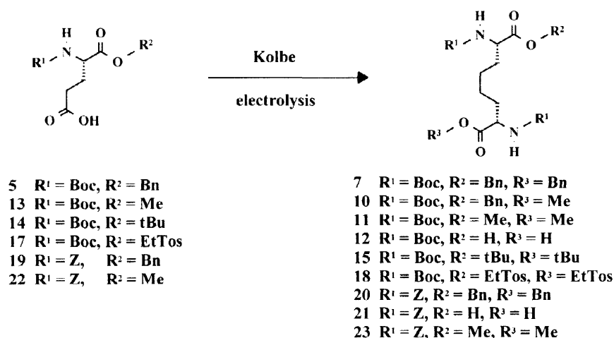
Scheme 3: Synthesis of 2,7-diaminosuberic acid derivatives by Kolbe electrolysis
